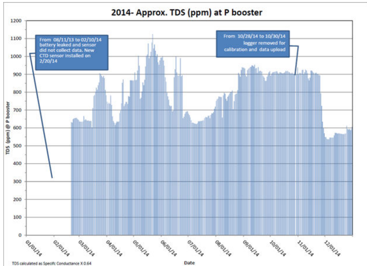
Figure 1 – Approximate TDS at P Booster (2014)
